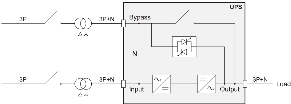
UPS with a separate bypass supply (option) connected to an independent supply and with galvanic isolation on the input
